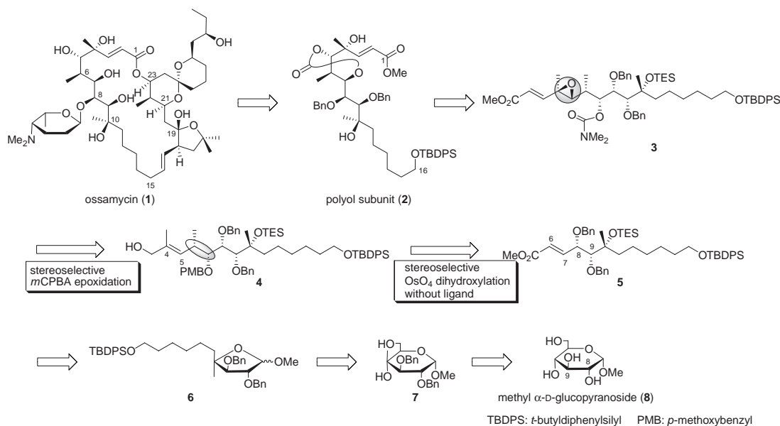
Scheme 1. Retrosynthetic analysis.
